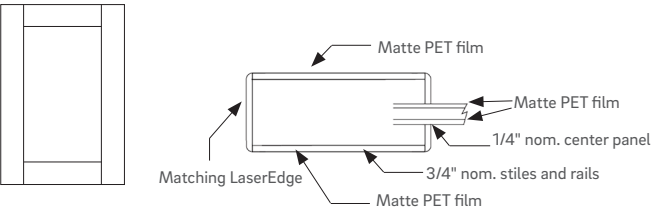
Shaker profile
